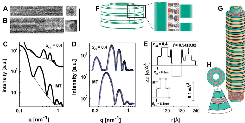
FIGURE 2 TEM images, SAXRD scans, and analysis of MTs and MTs complexed with DOTAP/DOPC membranes (see Materials and Methods). (A) TEM images of an MT. A whole-mount image is on the left side and a cross section is shown on the right. (B) TEM image of an LPN. The mole fraction of charged lipids, x_{\text{CL}} \equiv N_{\text{CL}} / (N_{\text{CL}} + N_{\text{NL}}) = 0.5 , and the cationic lipid/tubulin stoichiometry, R_{\text{CL/T}} \equiv N_{\text{CL}} / N_{\text{T}} = 120 . N_{\text{CL}} and N_{\text{NL}} are the numbers of cationic and neutral lipids, respectively, and N_{\text{T}} is the number of tubulin dimers. A whole mount image is on the left side and a cross section, showing an inner MT with 14 PFs, is on the right. We note that we did not perform a statistical study of such TEM cross section, as our
