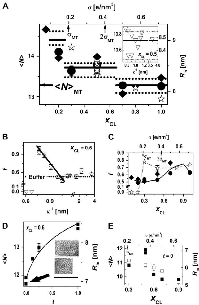
FIGURE 4 The effect of salt, taxol, and membrane spontaneous curvature and rigidity on the mean PF number, \langle N \rangle , and tubulin oligomer coverage, f . The cationic lipid/tubulin stoichiometry R_{CL/T} = 160 \cdot x_{CL} for all data points. (A) \langle N \rangle (or R_{in} ) as a function of x_{CL} (or \sigma ). The solid and broken lines are taken from Fig. 3 B, indicating the mean values of \langle N \rangle and the upper and lower limits of \langle N \rangle at each step, respectively, for MTs complexed with DOTAP/DOPC membranes. Solid diamonds indicate the \langle N \rangle values of MTs complexed with DLTAP/DLPC membranes and solid circles indicate the values for MTs complexed with DOTAP/DOPE membranes. Open symbols indicate the effect of added salt when MTs are complexed with DOTAP/DOPC membranes. Stars indicate the addition of 50 mM KCl (leading to Debye length of \kappa^{-1} = 0.9 nm, when the buffer is taken into account) at several membrane charge densities. Triangles indicate the addition of different salt concentrations when x_{CL} = 0.5 . The inset shows the variation of \langle N \rangle with \kappa^{-1} , when x_{CL} = 0.5 . (B) The variation of f with \kappa^{-1} (i.e., salt) for x_{CL} = 0.5 , for MTs complexed with DOTAP/DOPC membranes. The broken line indicates the mean value of f for the complexes in the buffer solution with no added salt. The solid line is a guide for the eye. (C) f as a function of x_{CL} . The solid line is taken from Fig. 3 A. Other symbols are as in Fig. 4 A. (D) \langle N \rangle (or R_{in} ) as a function of the molar ratio, t , between taxol and tubulin for x_{CL} = 0.5 with DOTAP/DOPC membranes. The solid line is a fit to a logarithmic expression: \langle N \rangle = \ln(142218 + 883725 \times t) . The inset is a TEM cross section (bottom) corresponding to t = 0 (arrow), showing the inner MT with 12 PFs and a TEM side-view image (top) showing a short LPN. (Scale bar, 50 nm.) We note that we did not perform a statistical study of such TEM cross sections, as our x-ray data is a bulk measurement and inherently includes statistics. (E) \langle N \rangle (or R_{in} ) as a function of x_{CL} (or \sigma ) for t = 0 , corresponding to no added taxol. Open squares correspond to tubulin,
