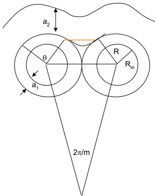
FIGURE 5 Cartoon demonstrating the geometry associated with a membrane that coats the MT PFs.
