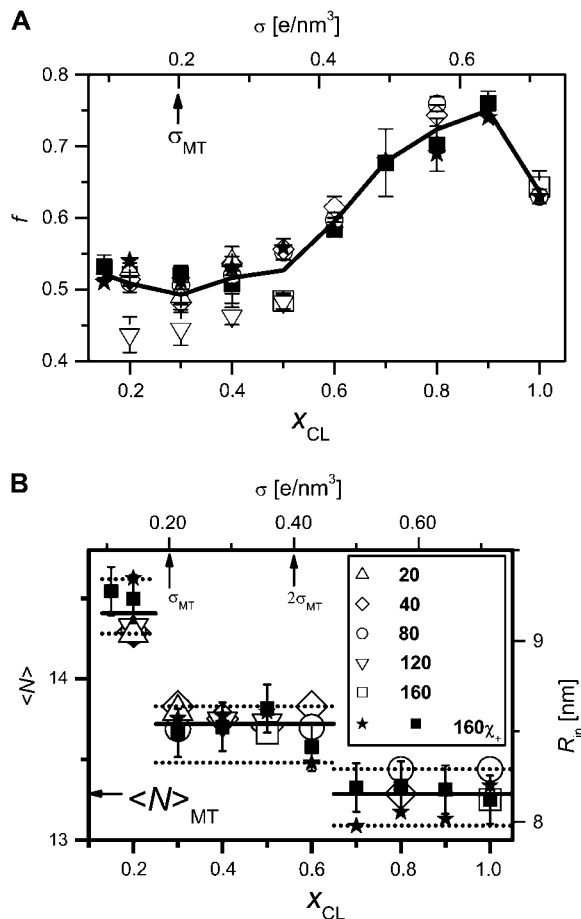
FIGURE 3 States diagrams of the LPNs as a function of the mole fraction of cationic lipids, x_{CL} , or the membrane charge density, \sigma (top horizontal axis); \sigma is calculated from x_{CL} as explained in Results and Discussion. The MT wall charge density, \sigma_{MT} , as estimated based on the primary structure of tubulin (15,16,31,40), is indicated. Each data point is obtained from scattering data and fitting to a model, as demonstrated in Fig. 2. Different symbols correspond to different charged lipid/tubulin ratios, R_{CL/T} , as indicated in Fig. 3 B (inset). For all data points shown, there are enough lipids to cover each MT with a bilayer. Solid symbols, for which R_{CL/T} = 160 \cdot x_{CL} , correspond to a series of data points at which the total number of lipids/tubulin is kept constant and is exactly enough to coat each MT with a bilayer (calculated as in May and Ben-Shaul (35)). (A) Fraction of tubulin oligomer coverage at the external layer, f , as a function of x_{CL} (or \sigma ). The solid line indicates the mean values of f(x_{CL}) . (B) The inner wall radius, R_{in} , of the internal MT within the LPN complex and mean PF number, \langle N \rangle , as a function of x_{CL} (or \sigma ). R_{in} is obtained from fitting the scattering data to the model, whereas \langle N \rangle is estimated from R_{in} (see Results and Discussion). The arrow indicates the \langle N \rangle value of pure MTs, \langle N \rangle_{MT} = 13.3 , as obtained from the fit to the MT form factor, shown in Fig. 2, in good agreement with earlier work (14,15,20,22). The three solid lines indicate the mean values of \langle N \rangle at each step. The broken lines indicate the maximum and the minimum values of \langle N \rangle at each step.
