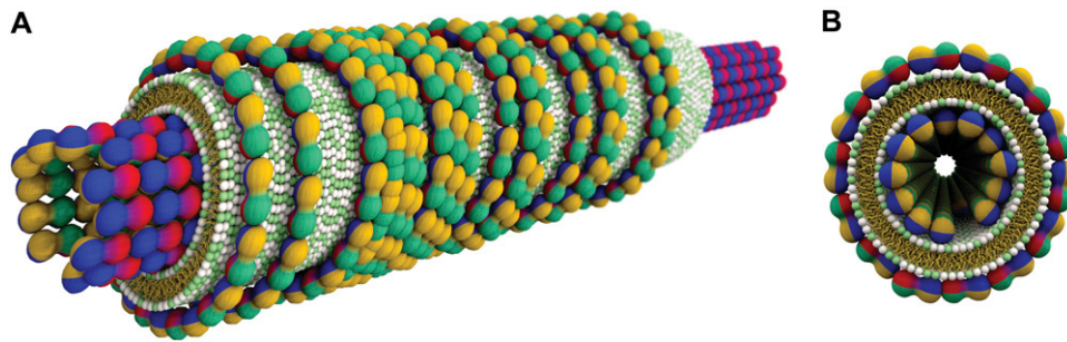
FIGURE 1 (A) A side-view cartoon of the LPN structure showing a microtubule made of tubulin protein subunits (red-blue-yellow-green objects) coated by a lipid bilayer (with yellow tails and green/white headgroups), which in turn is coated by a third layer of tubulin oligomers exposing the side that in MT is facing the lumen. (B) A top-view cartoon of the LPN structure.
