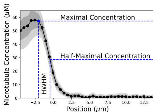
Figure E1. Illustration of the procedure for defining a HWHM for the interface from the data. We measure the distance at which the microtubule concentration has decayed to half the value it had at the first point from which the concentration profile started decaying.
