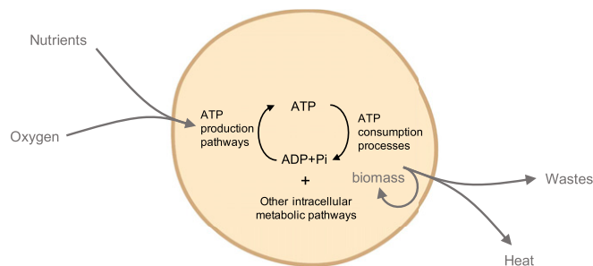
Fig. 2. Schematic of typical cellular chemical and energy fluxes. Energy fluxes represent the conversion rate of Gibbs energy derived from the environment, e.g. from nutrients, through cellular activities to waste products, biomass, or heat. Gray arrows represent the global energy flux through the cell. The enthalpic part of the global energy flux can be measured as the heat production rate of the cell. For aerobic organisms, measurements of the OCR can be related to the rate of heat production through Thornton's rule (46). Intracellular energy fluxes are represented by the fluxes through specific metabolic pathways, such as those that produce and consume ATP.
